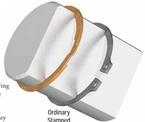
Smalley® Spiral Retaining Ring
